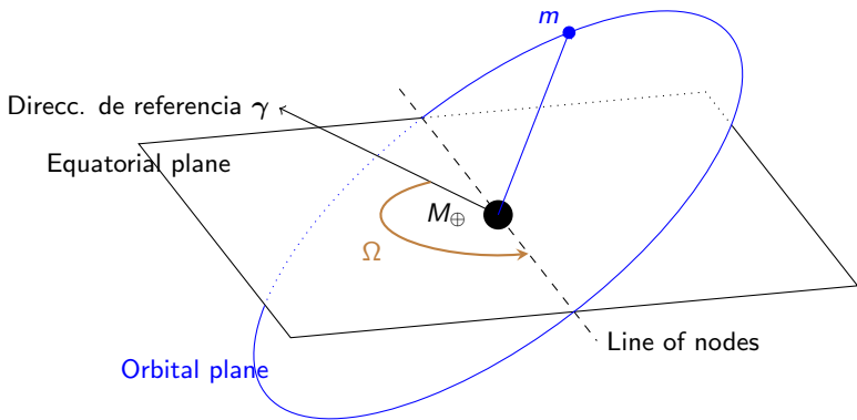
Figure: Orbital elements or Keplerian elements
